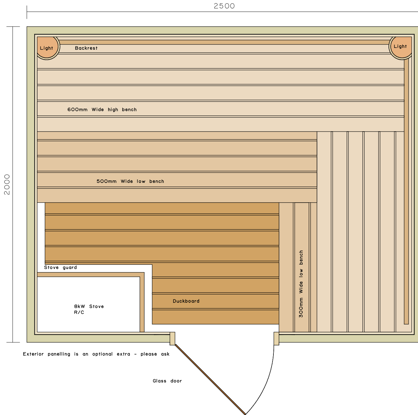
Suggested Sauna Layout - Scale 1:15 Optimum Sauna ceiling height 2150mm
