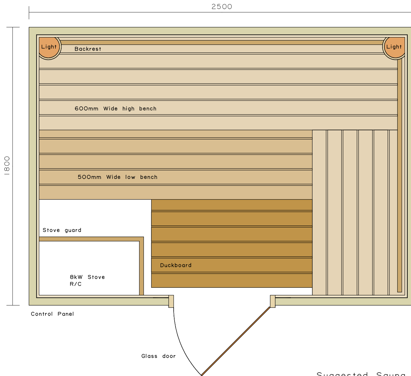
Suggested Sauna Layout - Scale 1:15 Optimum Sauna ceiling height 2150mm
