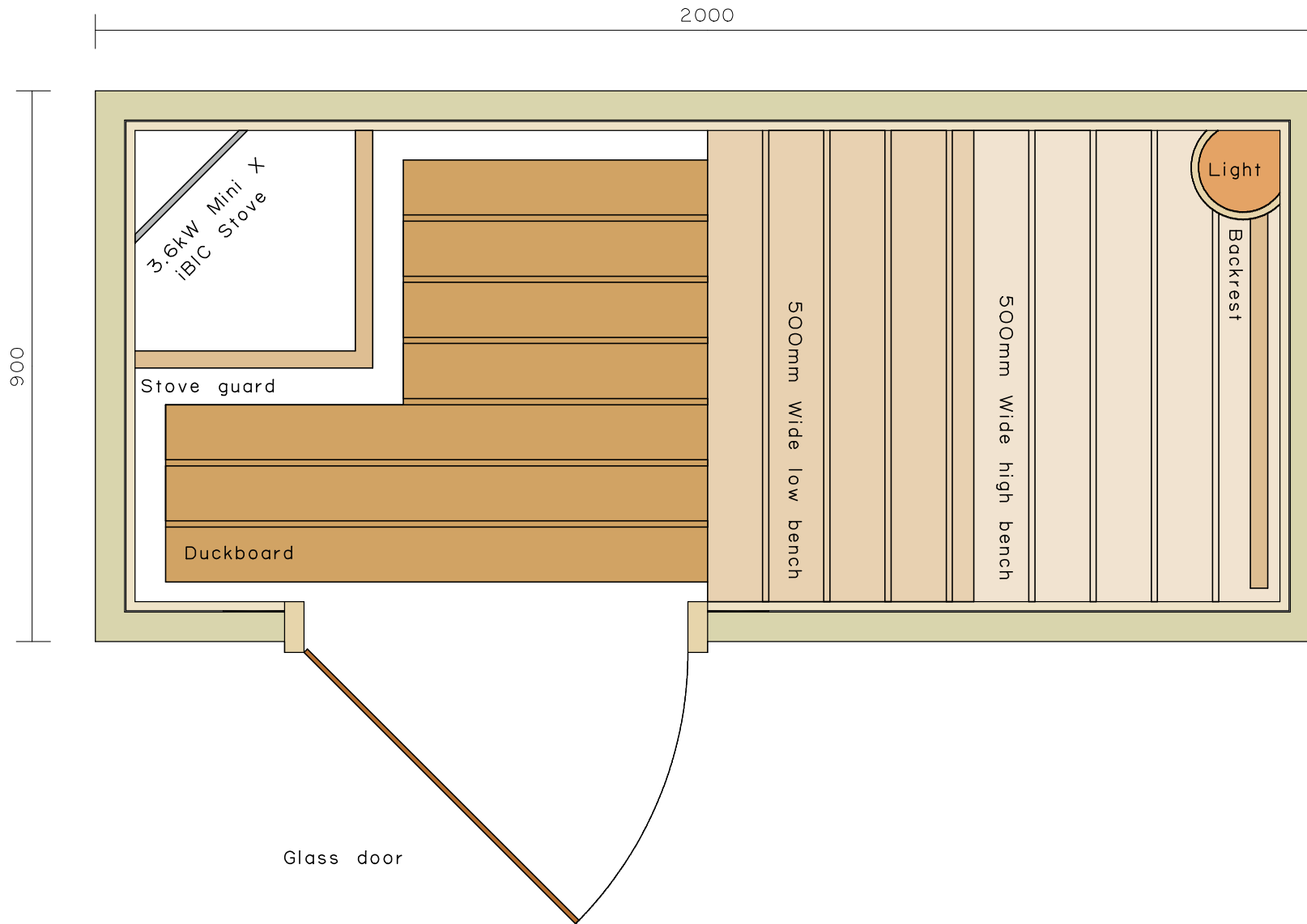
Suggested Sauna Layout - Scale 1:10 Optimum Sauna ceiling height 2150mm
