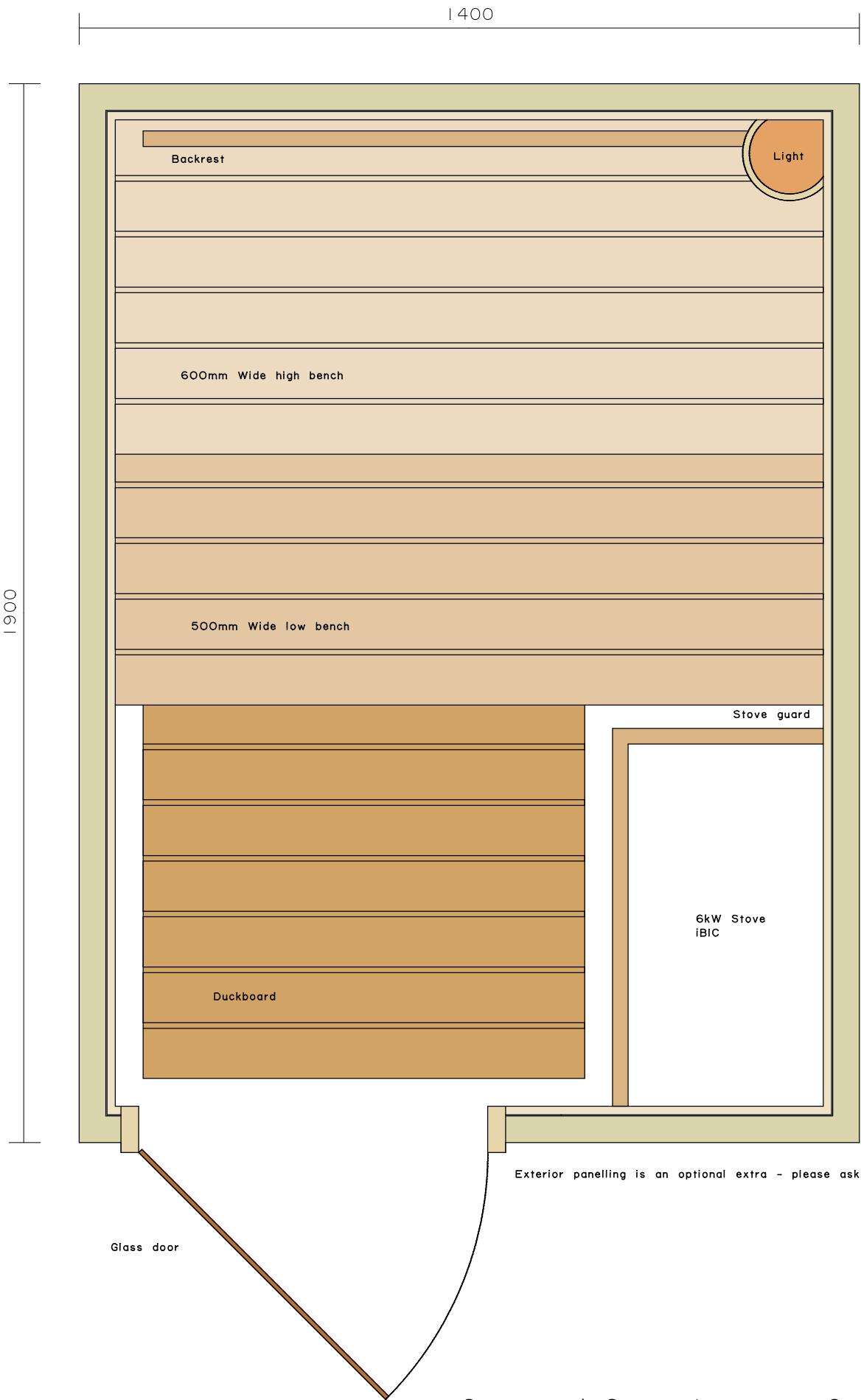
Suggested Sauna Layout - Scale 1:10 Optimum Sauna ceiling height 2150mm
