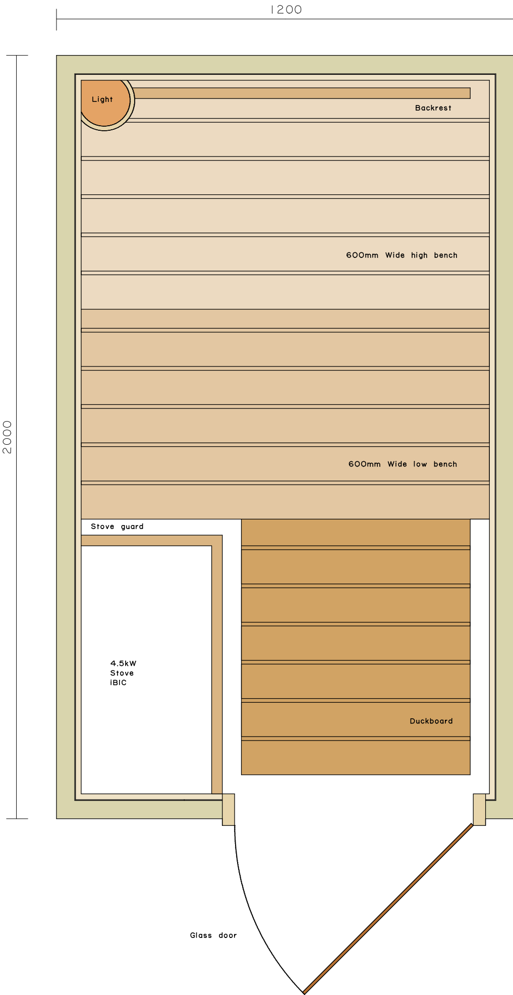
Suggested Sauna Layout - Scale 1:10 Optimum Sauna ceiling height 2150mm
