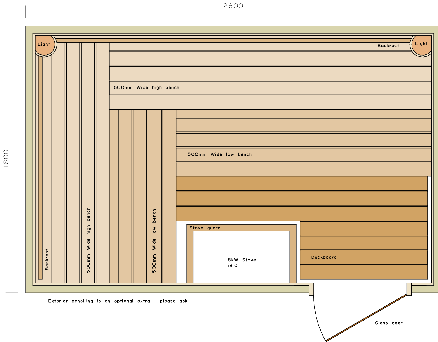
Suggested Sauna Layout - Scale 1:15 Optimum Sauna ceiling height 2150mm
