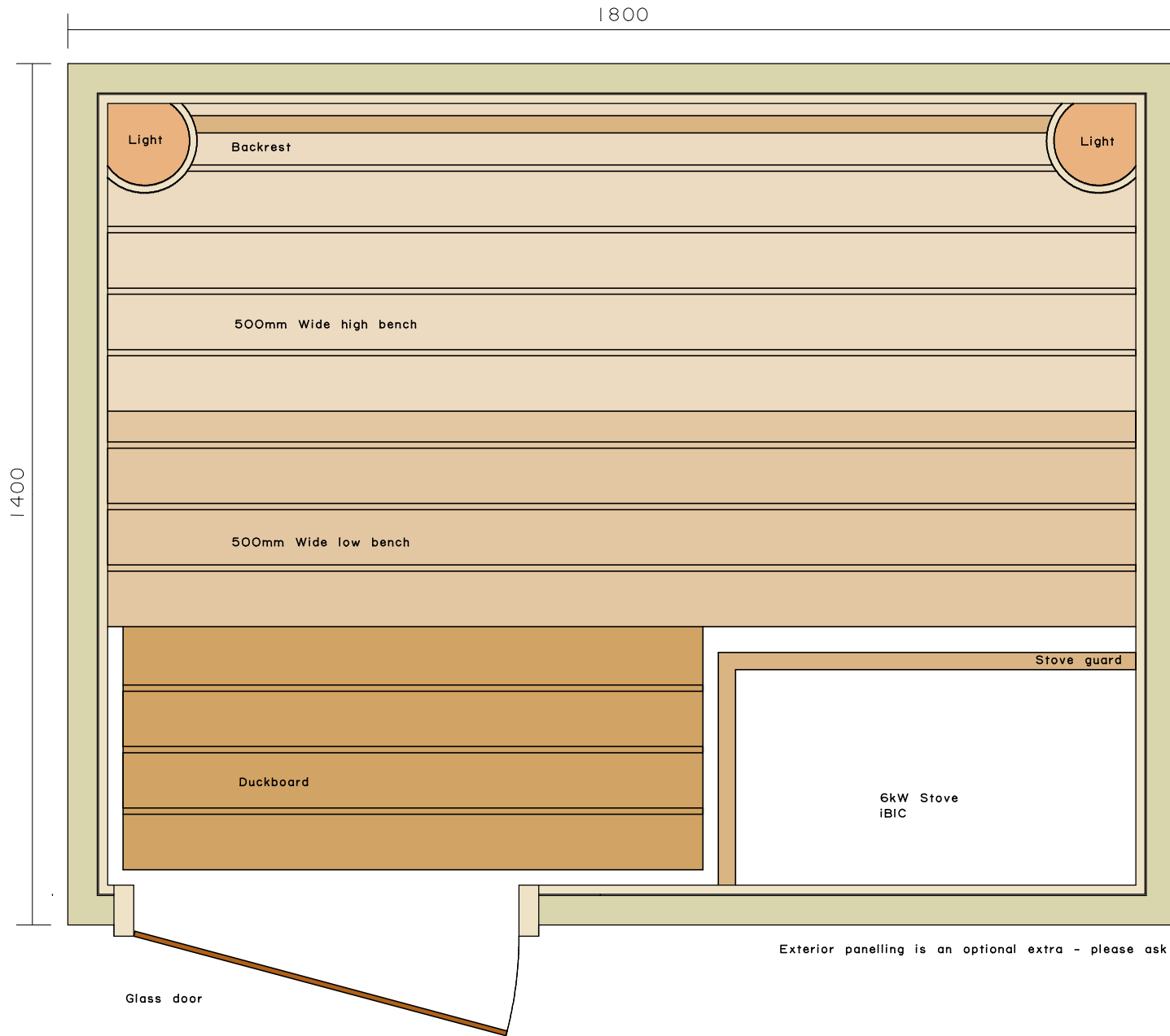
Suggested Sauna Layout - Scale 1:10 Optimum Sauna ceiling height 2150mm
