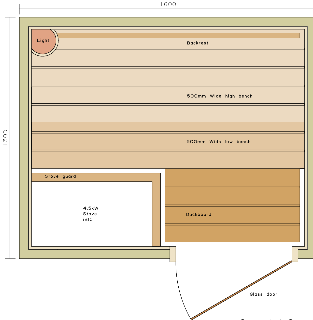
Suggested Sauna Layout - Scale 1:10 Optimum Sauna ceiling height 2150mm
