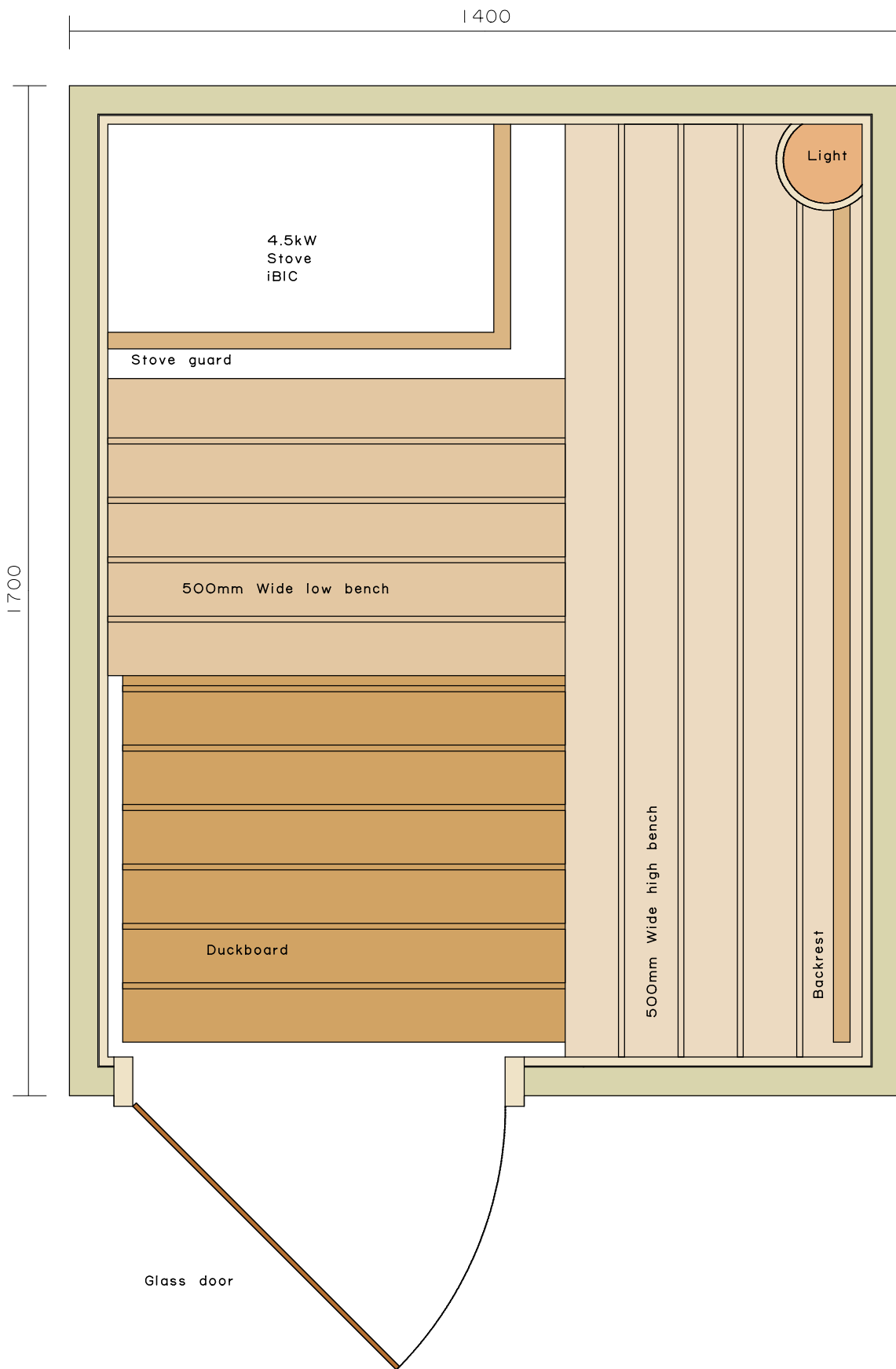
Suggested Sauna Layout - Scale 1:10 Optimum Sauna ceiling height 2150mm
