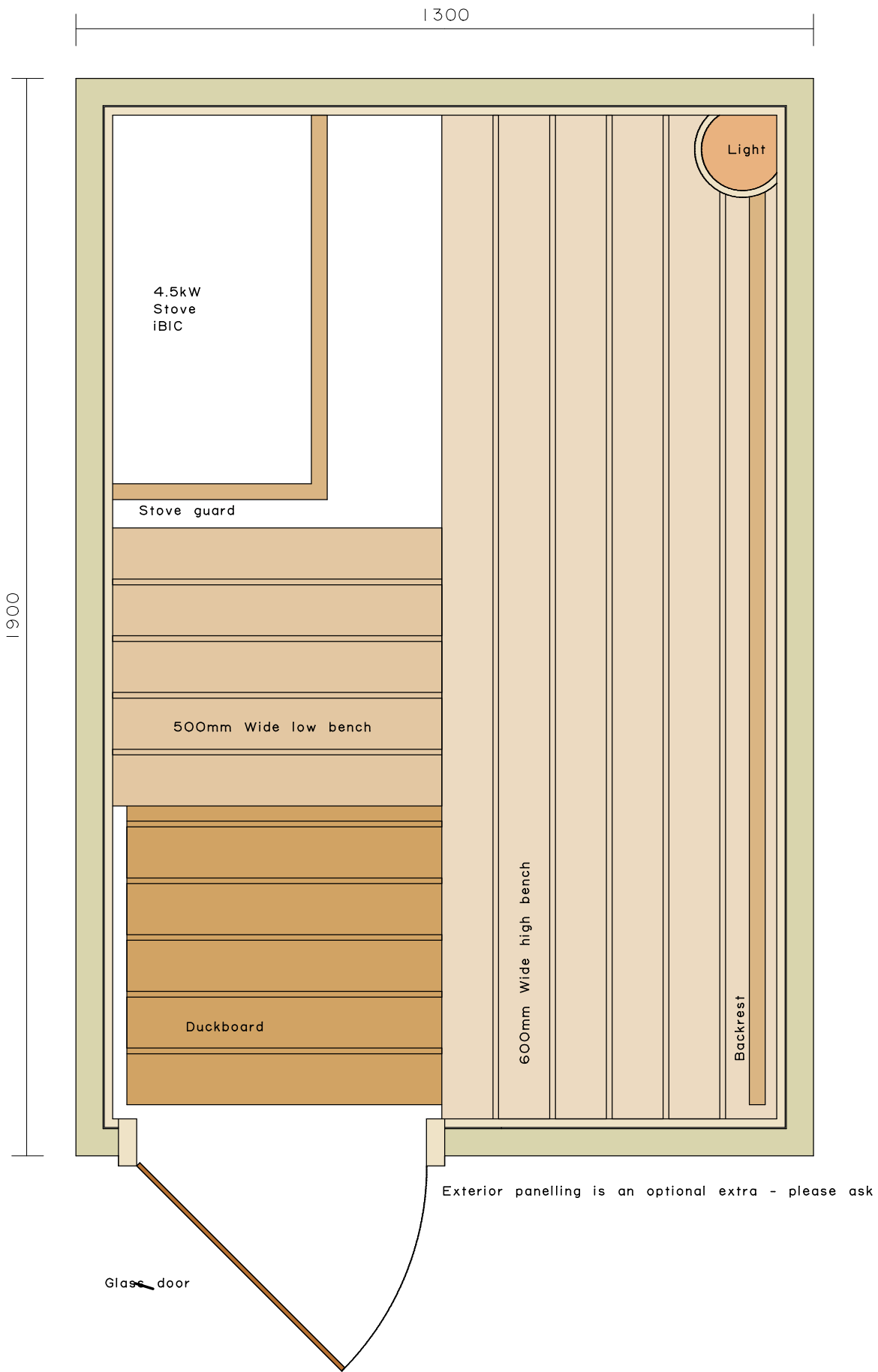
Suggested Sauna Layout - Scale 1:10 Optimum Sauna ceiling height 2150mm
