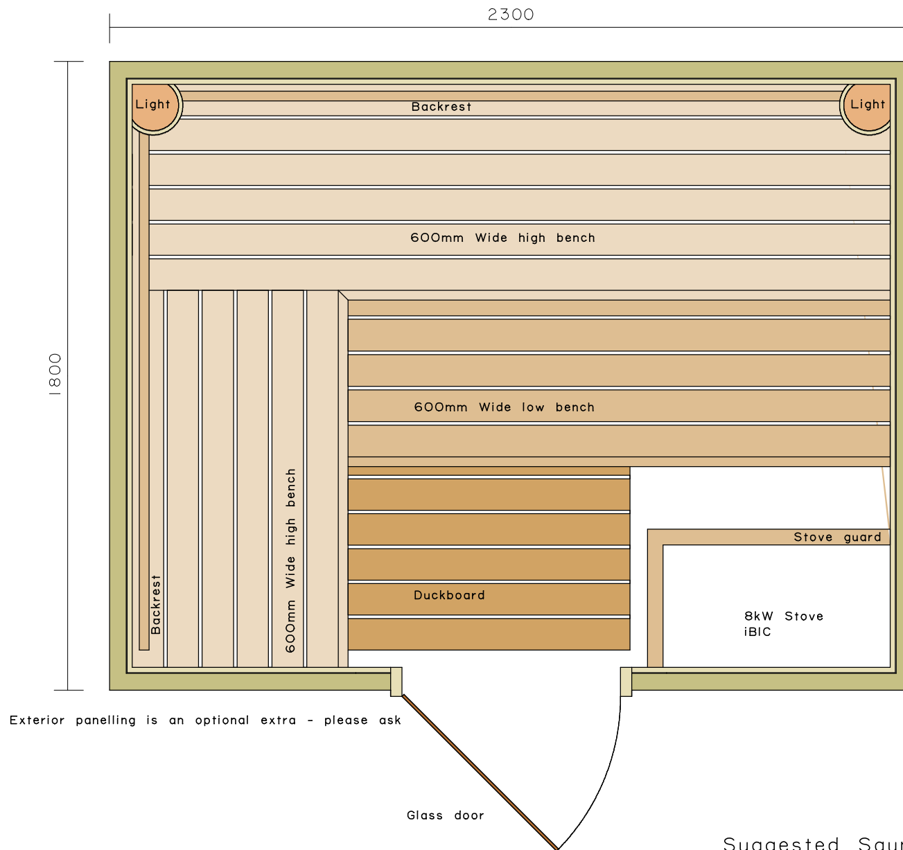
Suggested Sauna Layout - Scale 1:15 Optimum Sauna ceiling height 2150mm
