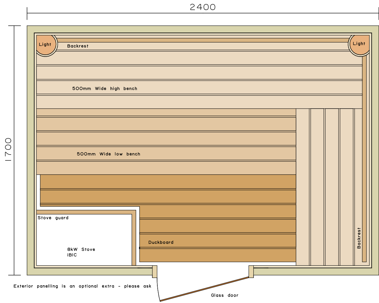
Suggested Sauna Layout - Scale 1:15 Optimum Sauna ceiling height 2150mm
