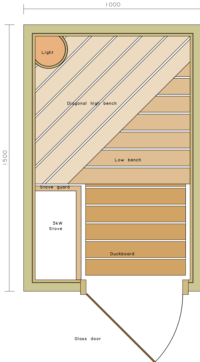
Suggested Sauna Layout - Scale 1:10 Optimum Sauna ceiling height 2150mm
