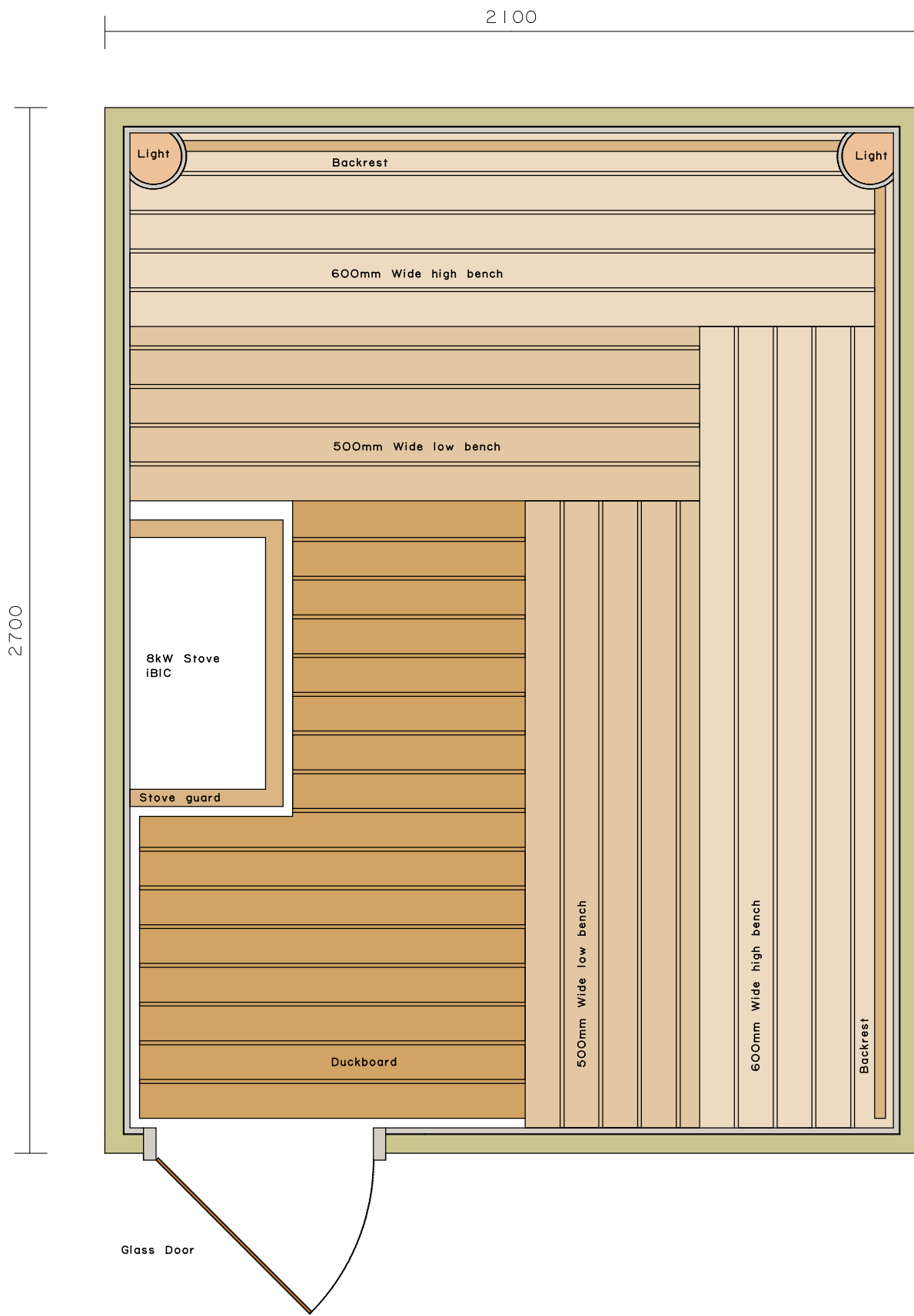
Suggested Sauna Layout - Scale 1:15 Optimum Sauna ceiling height 2150mm
