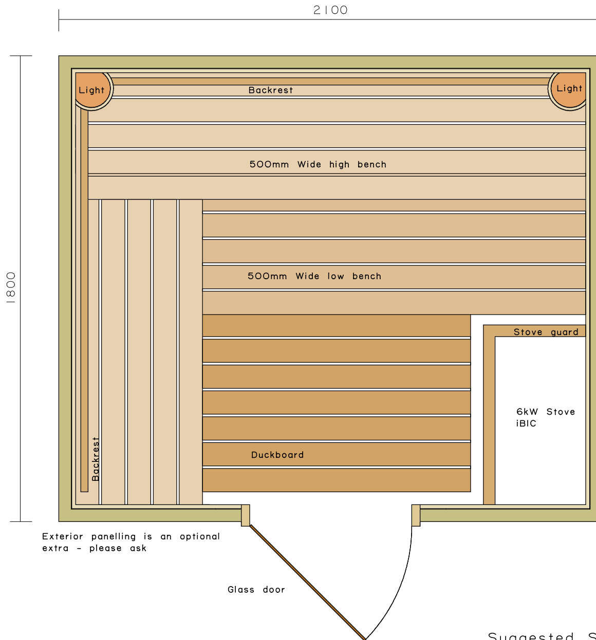
Suggested Sauna Layout - Scale 1:15 Optimum Sauna ceiling height 2150mm
