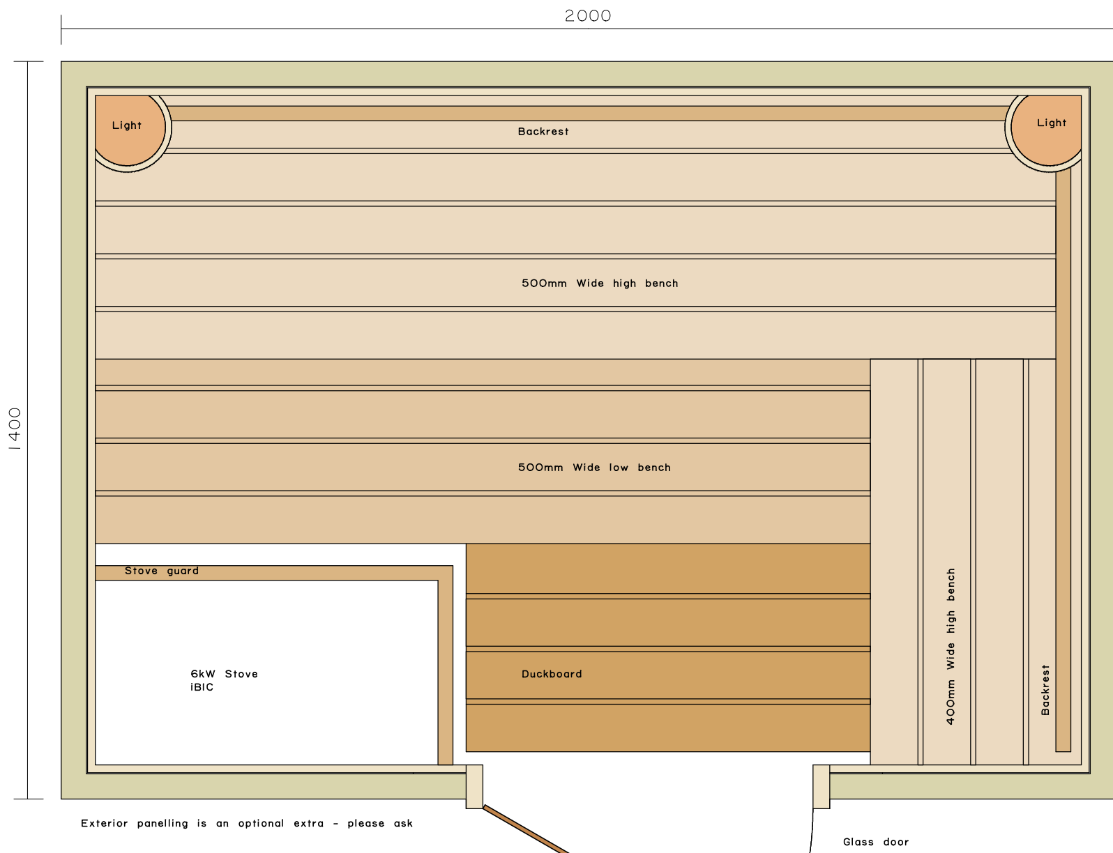
Suggested Sauna Layout - Scale 1:10 Optimum Sauna ceiling height 2150mm
