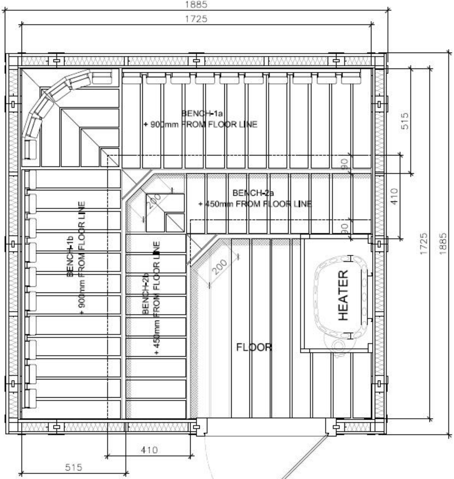
Sawo 'Sulu' 1919RL - with SCA-60NBUK Stove
