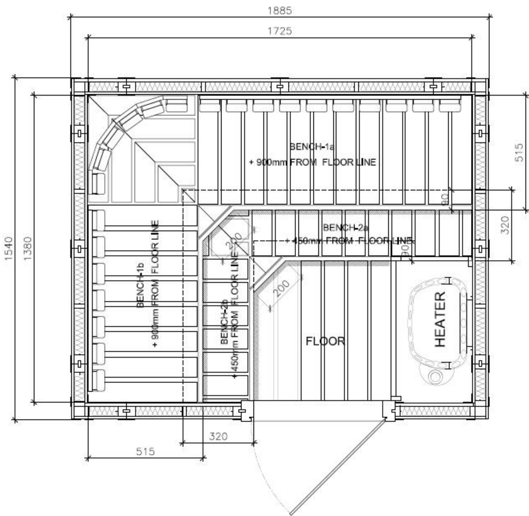
Sulu 1519RL - with SCA-60NBUK Stove
